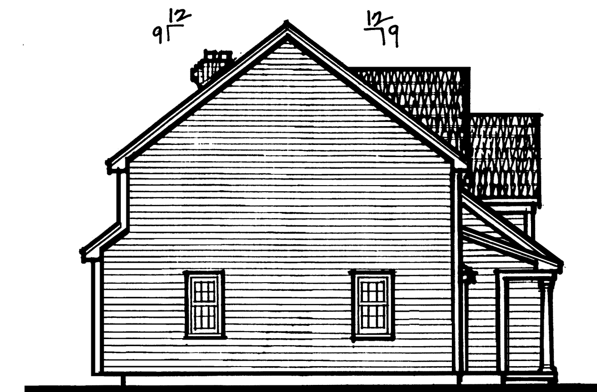
LEFT SIDE ELEVATION \frac{1}{8}'' = 1'-0''
