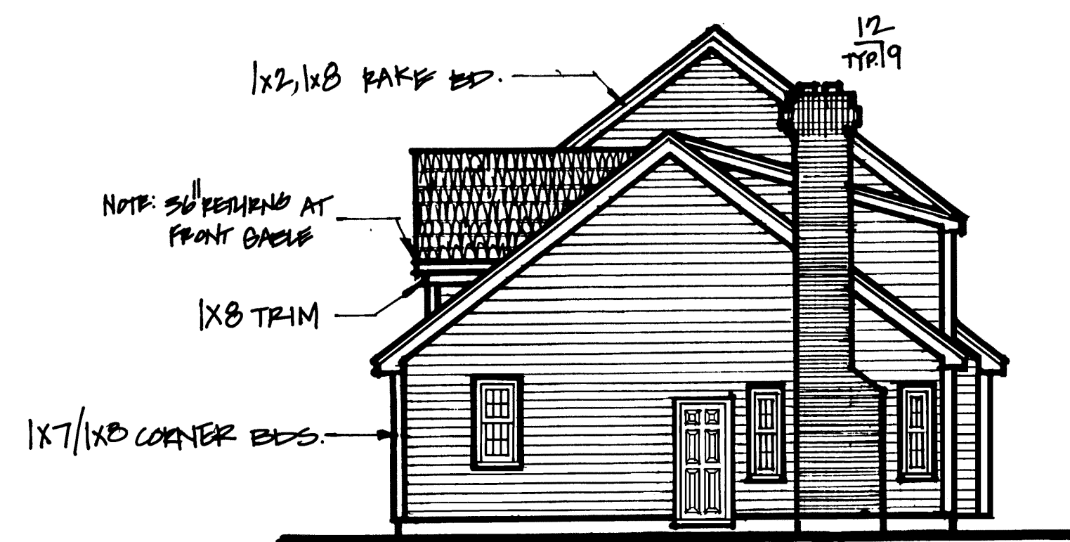
RIGHT SIDE ELEVATION \frac{1}{8}'' = 1'-0''
