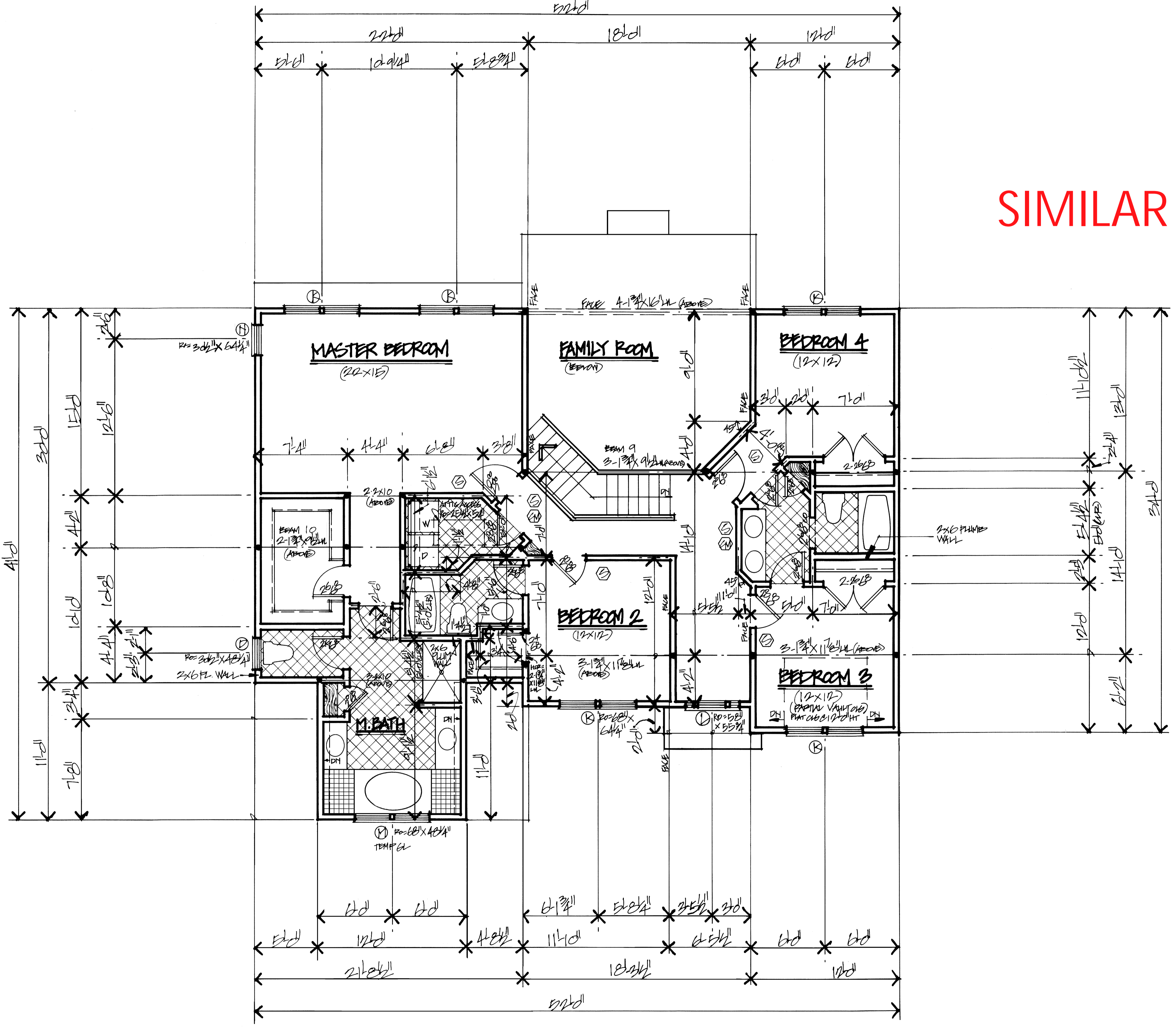
SECOND FLOOR PLAN 1/4" = 1'-0"
